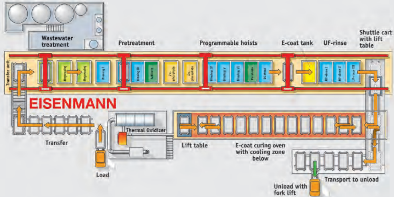
Indexing system with programmable hoist and roller conveyors connecting load and unload stations.
