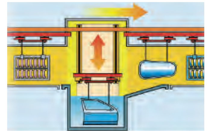
Diagram of an indexing system with power & free conveyor.
